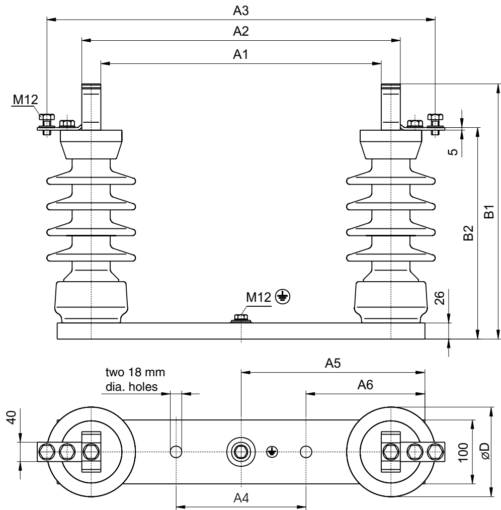
Dimensional drawing of PBWMNIII 36 w.II-1 type fuse-bases
